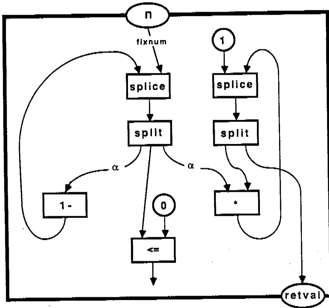
Figure 1 - The Dataflow Graph for ifact .
