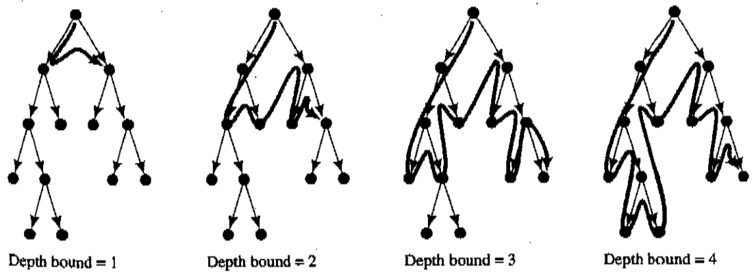
Figure 8.5 Stages in Iterative-Deepening Search
