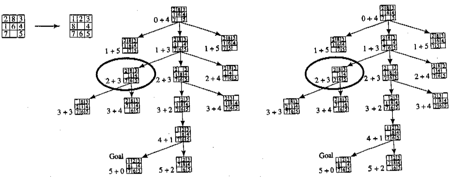
Figure 8.5 Stages in Iterative-Deepening Search
